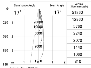
■ Direct Horizontal Illuminance DD155-1515WW9027
