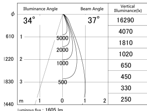
■ Direct Horizontal Illuminance DD155-1535WW9027
