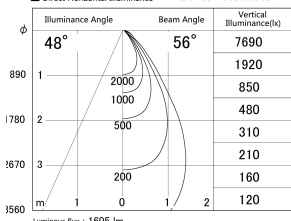
■ Direct Horizontal Illuminance DD155-1555WW9027
