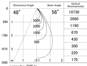
■ Direct Horizontal Illuminance DD155-2055WW9027
