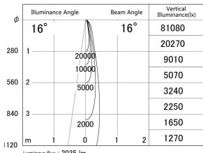
■ Direct Horizontal Illuminance DD155-2515WW9027
