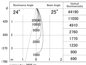
■ Direct Horizontal Illuminance DD155-2525WW9027
