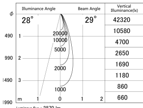
■ Direct Horizontal Illuminance DD155-2530WW9027
