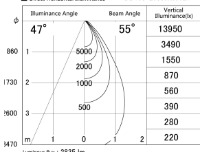
■ Direct Horizontal Illuminance DD155-2555WW9027
