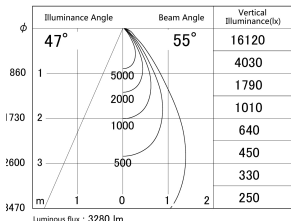
■ Direct Horizontal Illuminance DD155-3055WW9027
