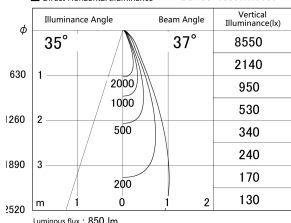
■ Direct Horizontal Illuminance DD155-0835WW9030
