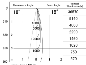
■ Direct Horizontal Illuminance DD155-1015WW9030
