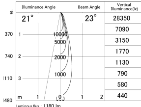
■ Direct Horizontal Illuminance DD155-1025WW9030
