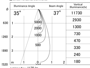
■ Direct Horizontal Illuminance DD155-1035WW9030
