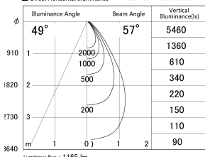
■ Direct Horizontal Illuminance DD155-1055WW9030
