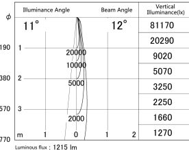
■ Direct Horizontal Illuminance DD155-1510WW9030
