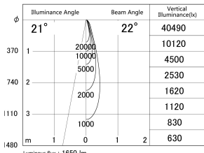
■ Direct Horizontal Illuminance DD155-1525WW9030
