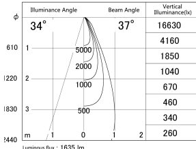
■ Direct Horizontal Illuminance DD155-1535WW9030
