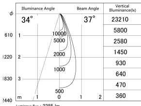
■ Direct Horizontal Illuminance DD155-2035WW9030
