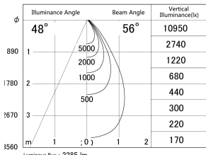
■ Direct Horizontal Illuminance DD155-2055WW9030
