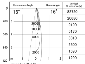
■ Direct Horizontal Illuminance DD155-2515WW9030
