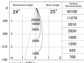
■ Direct Horizontal Illuminance DD155-2525WW9030
