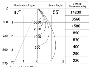
■ Direct Horizontal Illuminance DD155-2555WW9030
