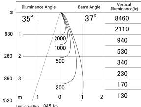
■ Direct Horizontal Illuminance DD155-0835WW9035
