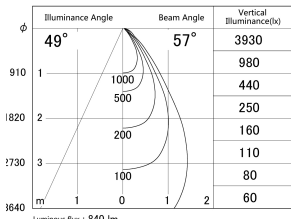
■ Direct Horizontal Illuminance DD155-0855WW9035
