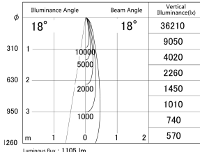
■ Direct Horizontal Illuminance DD155-1015WW9035
