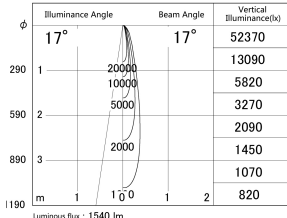
■ Direct Horizontal Illuminance DD155-1515WW9035
