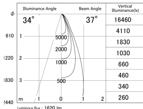
■ Direct Horizontal Illuminance DD155-1535WW9035
