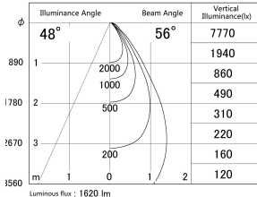
■ Direct Horizontal Illuminance DD155-1555WW9035
