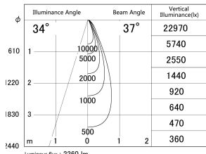
■ Direct Horizontal Illuminance DD155-2035WW9035
