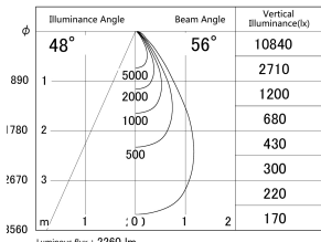
■ Direct Horizontal Illuminance DD155-2055WW9035
