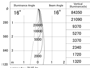
■ Direct Horizontal Illuminance DD155-2515WW9035
