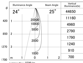
■ Direct Horizontal Illuminance DD155-2525WW9035
