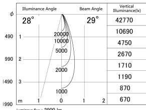
■ Direct Horizontal Illuminance DD155-2530WW9035
