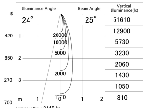
■ Direct Horizontal Illuminance DD155-3025WW9035
