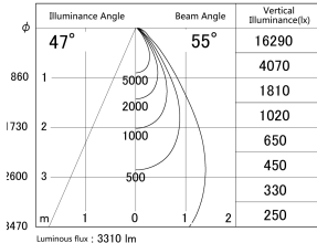
■ Direct Horizontal Illuminance DD155-3055WW9035
