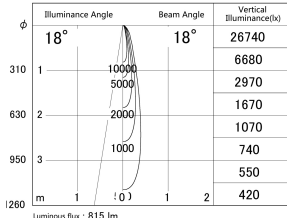
■ Direct Horizontal Illuminance DD155-0815WW9040
