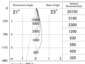
■ Direct Horizontal Illuminance DD155-0825WW9040
