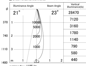
■ Direct Horizontal Illuminance DD155-1025WW9040
