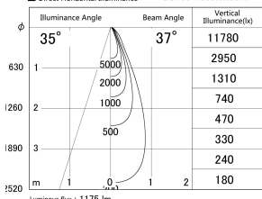
■ Direct Horizontal Illuminance DD155-1035WW9040
