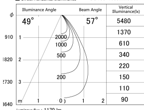
■ Direct Horizontal Illuminance DD155-1055WW9040
