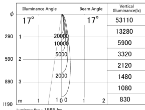
■ Direct Horizontal Illuminance DD155-1515WW9040
