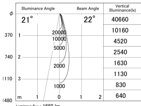
■ Direct Horizontal Illuminance DD155-1525WW9040
