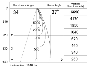
■ Direct Horizontal Illuminance DD155-1535WW9040
