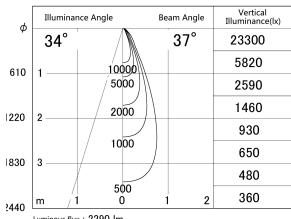
■ Direct Horizontal Illuminance DD155-2035WW9040
