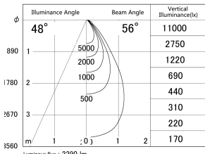
■ Direct Horizontal Illuminance DD155-2055WW9040
