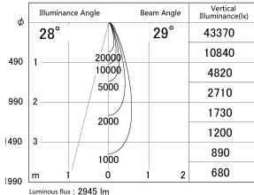
■ Direct Horizontal Illuminance DD155-2530WW9040
