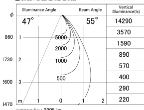
■ Direct Horizontal Illuminance DD155-2555WW9040
