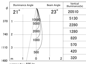
■ Direct Horizontal Illuminance DD155-0825MW9027-FX
