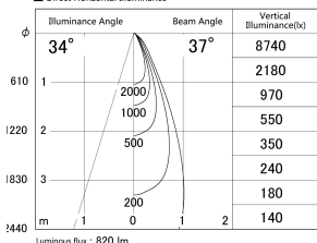
■ Direct Horizontal Illuminance DD155-0835MW9027-FX
