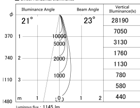
■ Direct Horizontal Illuminance DD155-1025MW9027-FX
